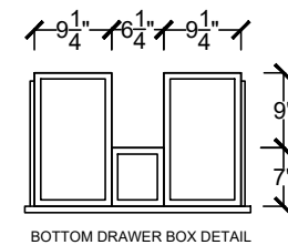
BOTTOM DRAWER BOX DETAIL
