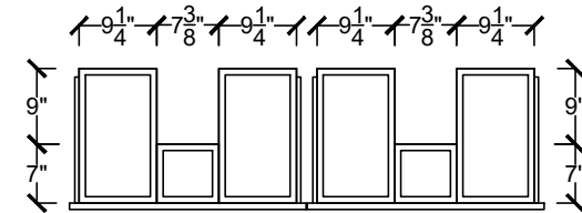
BOTTOM DRAWER BOX DETAILS
