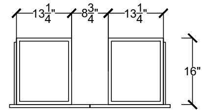
BOTTOM DRAWER BOX DETAIL
