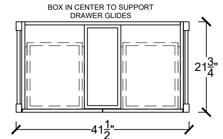
BOTTOM CABINET FLOOR DETAIL
