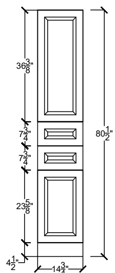
H-LINTC 1522-2D-
