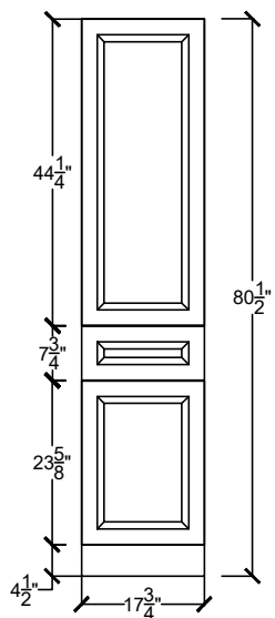
H-LINTC 1822-1D-
