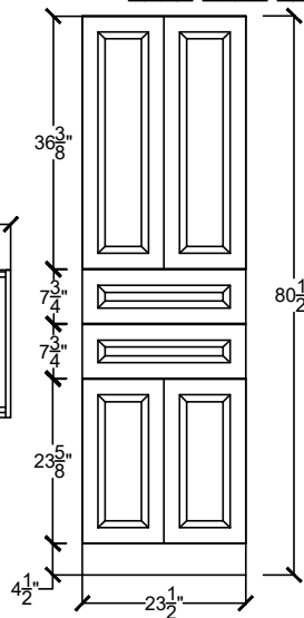
H-LINTC 2422-2D-
