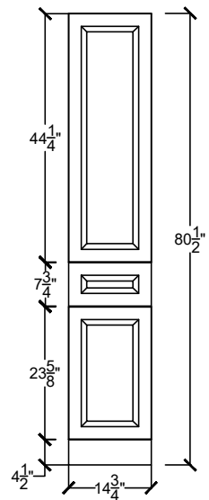
H-LINTC 1522-1D-
