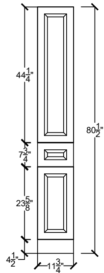
H-LINTC 1222-1D-
