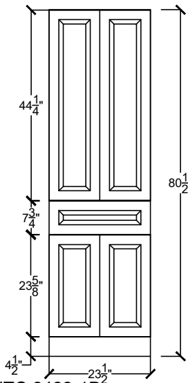
H-LINTC 2422-1D-
