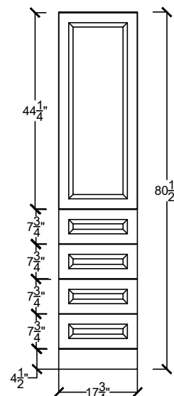
H-LINTC 1822-4D-
