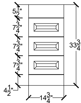
H-LINS 1522-3D- _____ - _____ - _____
