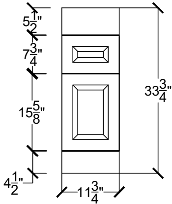
H-LINS 1222-1D- _____ - _____ - _____
